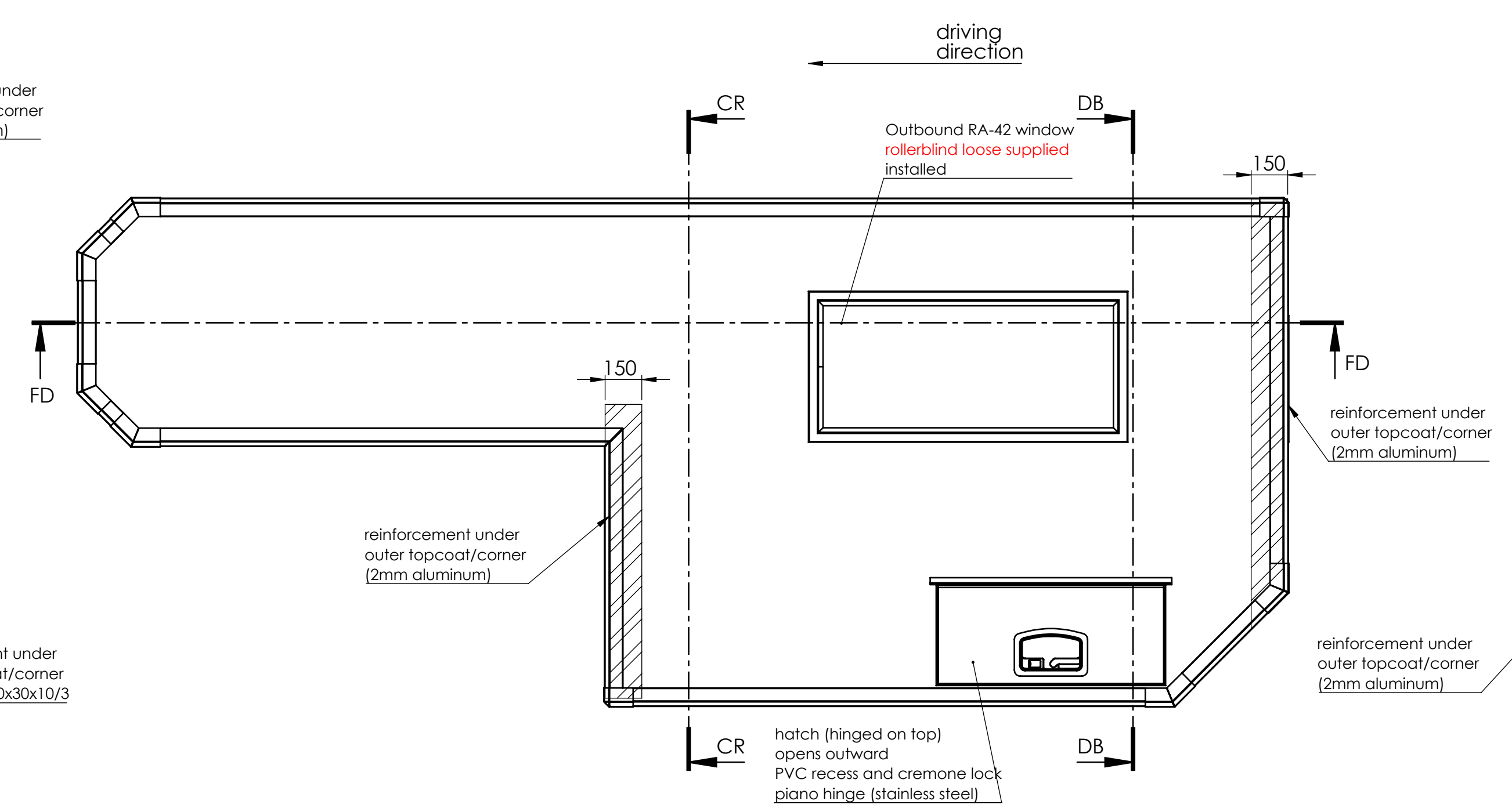
SCHNITT FD-FD view under roof
