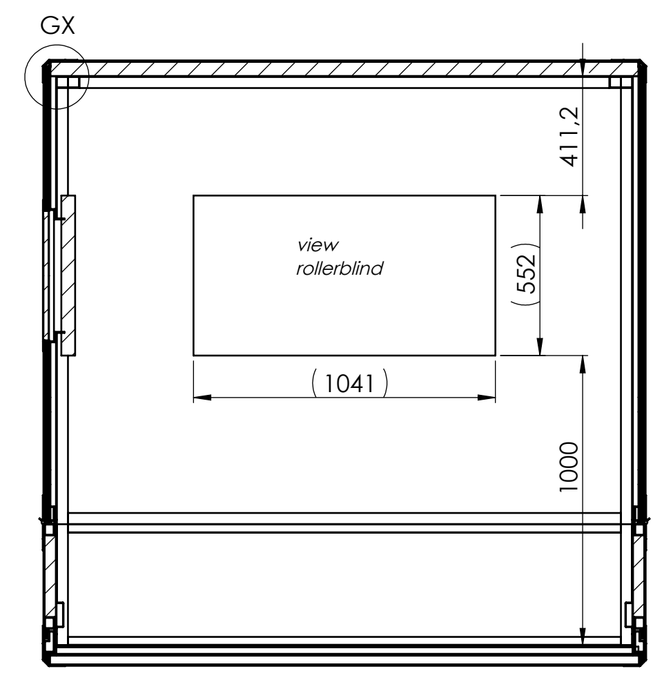
SCHNITT DB-DB view rear wall inside
