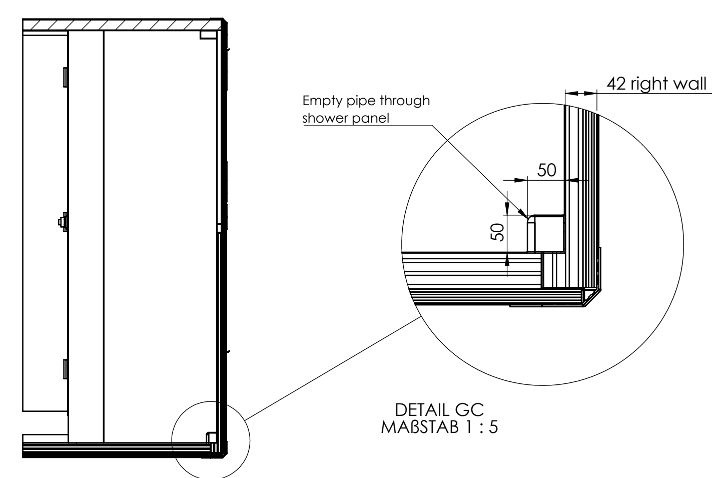
SCHNITT GA-GA view on wet bath (in driving direction)
