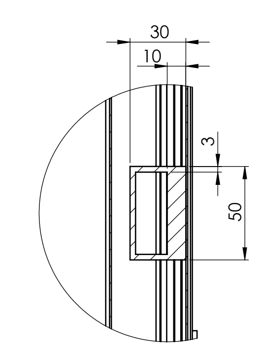
DETAIL GY MAßSTAB 1 : 2 aluminum square bar in rear wall
