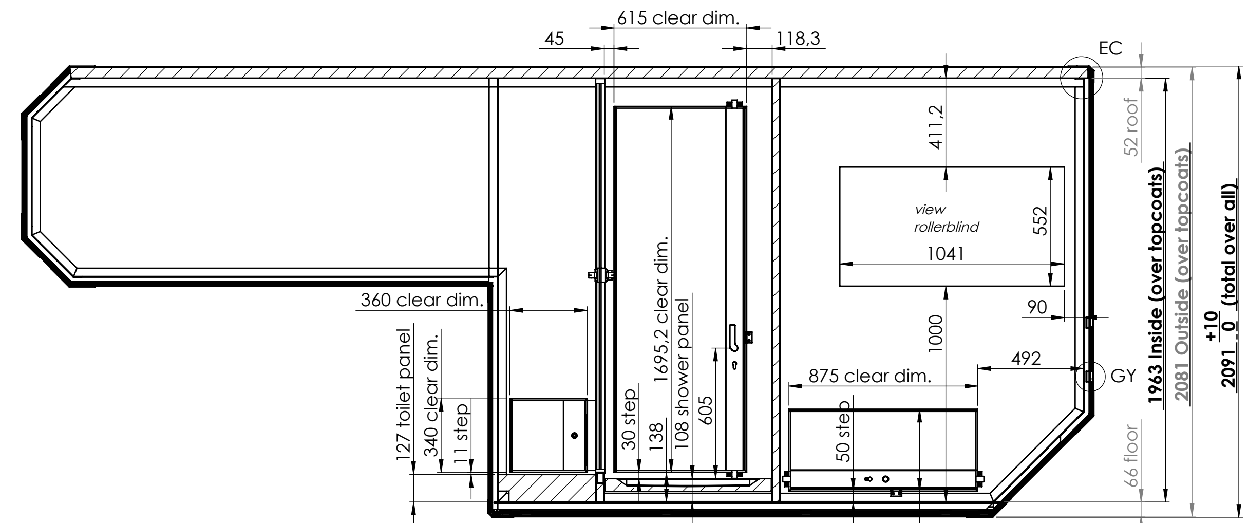
SCHNITT B-B view rear wall inside
